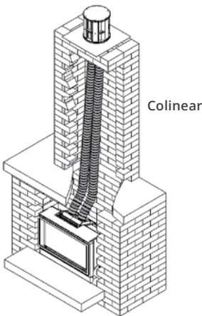
Direct Vent
